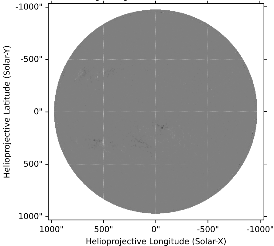
HMI magnetogram 2011-06-07 06:32:11
